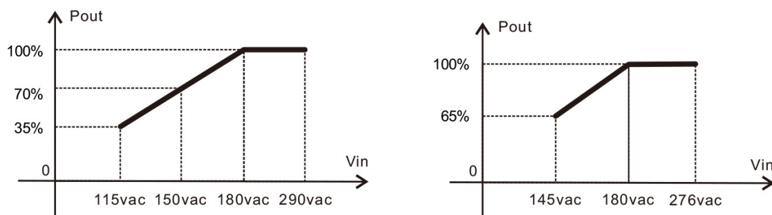
Figure 10 - Load Curve
