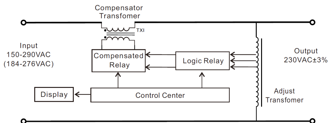
Figure 1 - Block Diagram of Electric Stabilizer
